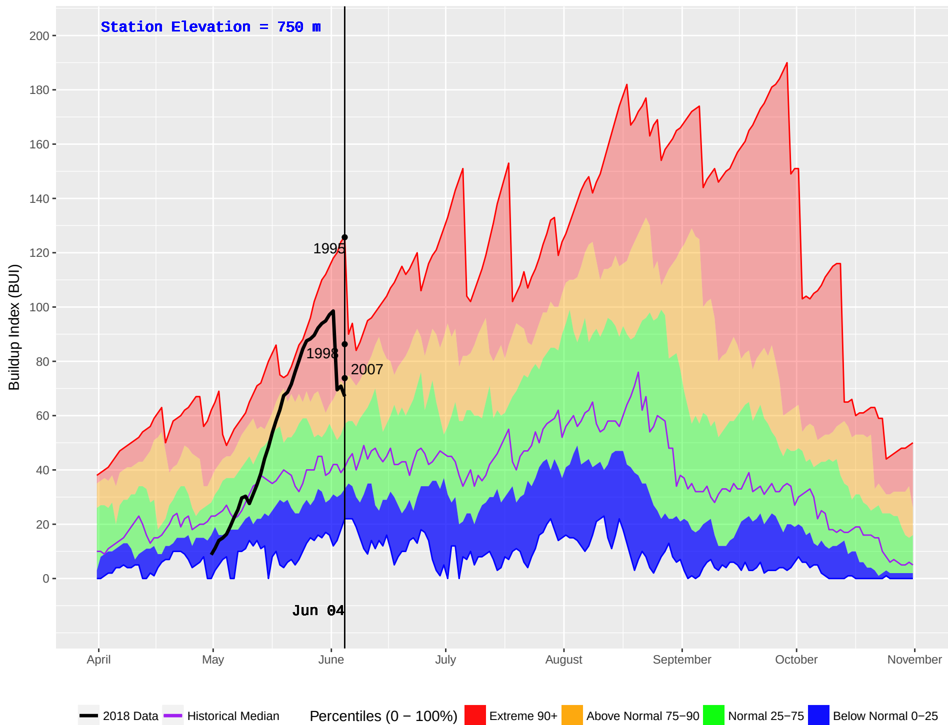
FORT ST JAMES (146) : Historical (1979–2016) and Current (2018) Noon Buildup Index (BUI)
