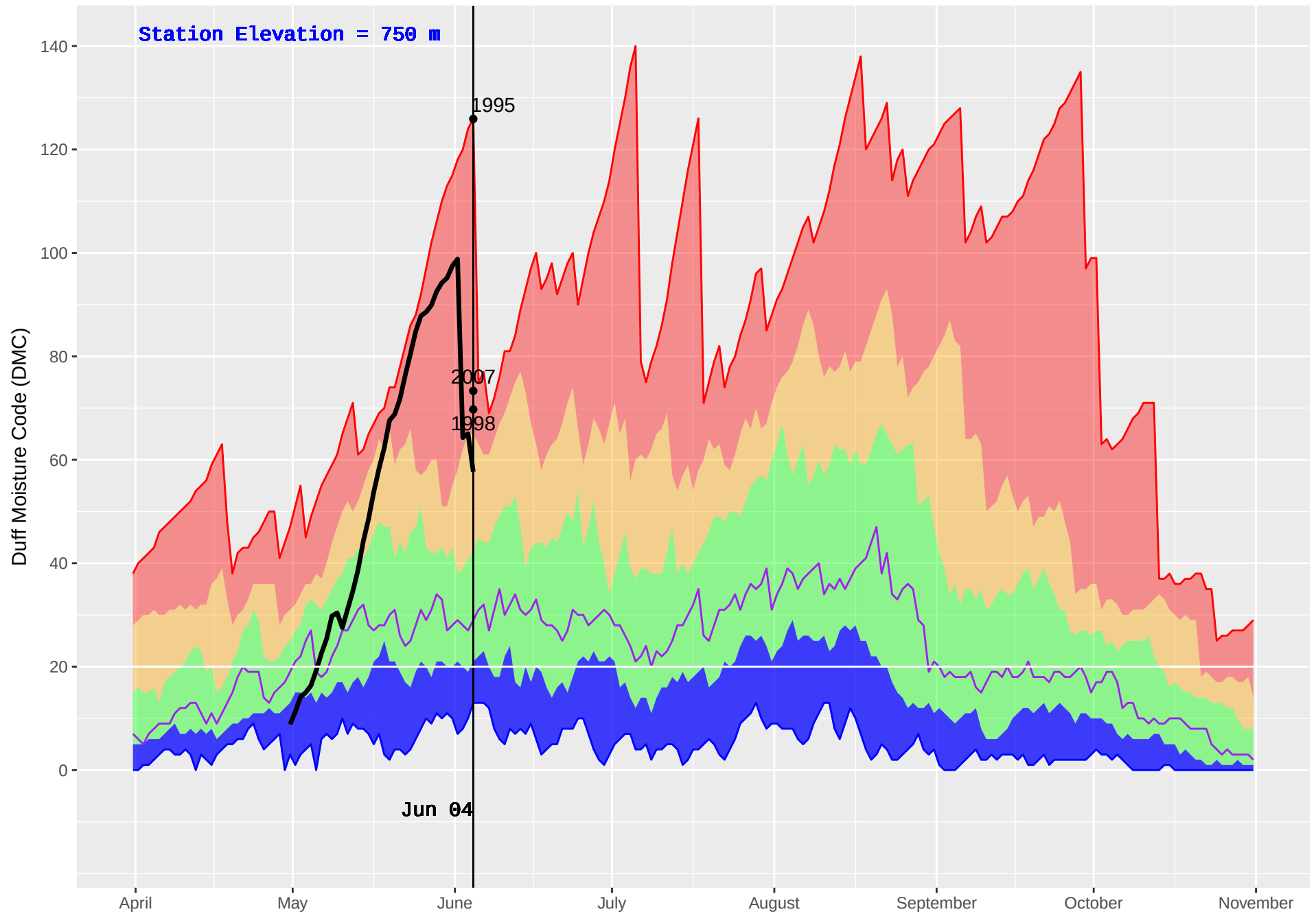
FORT ST JAMES (146) : Historical (1979–2016) and Current (2018) Noon Duff Moisture Code (DMC)
